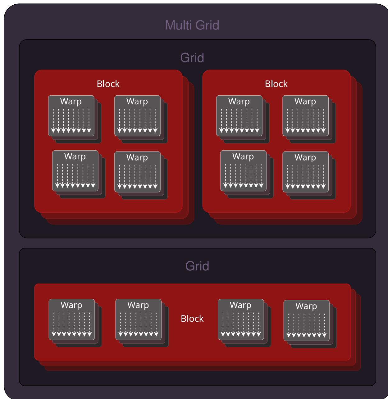
Fig. 8: Cooperative group thread hierarchy in grids.
