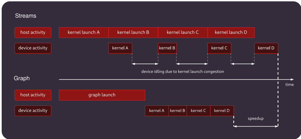
Fig. 10: Qualitative presentation of the execution time of many short-running kernels when launched using HIP stream versus HIP graph. This does not include the time needed to set up the graph.
