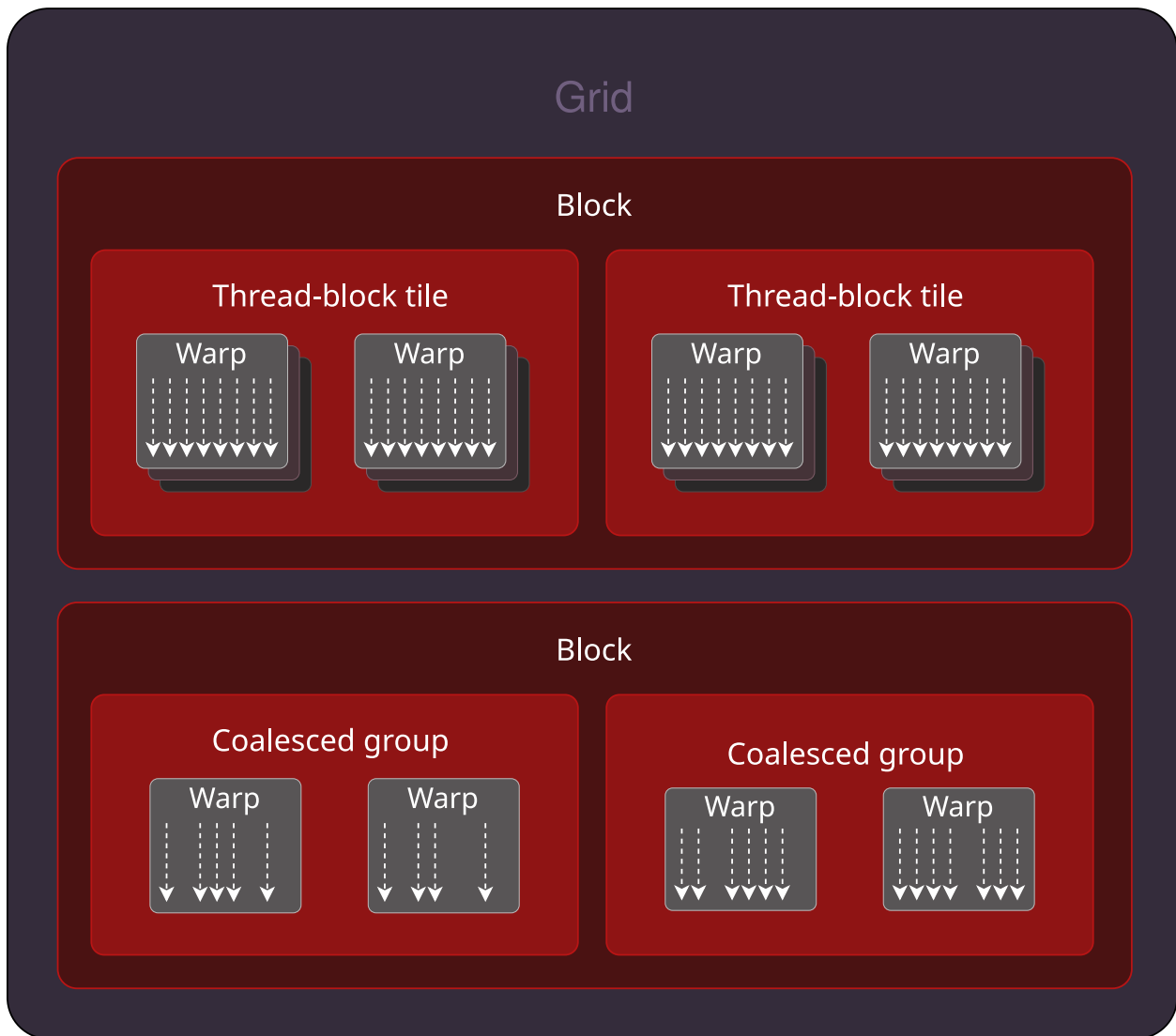
Fig. 9: Cooperative group thread hierarchy in blocks.
