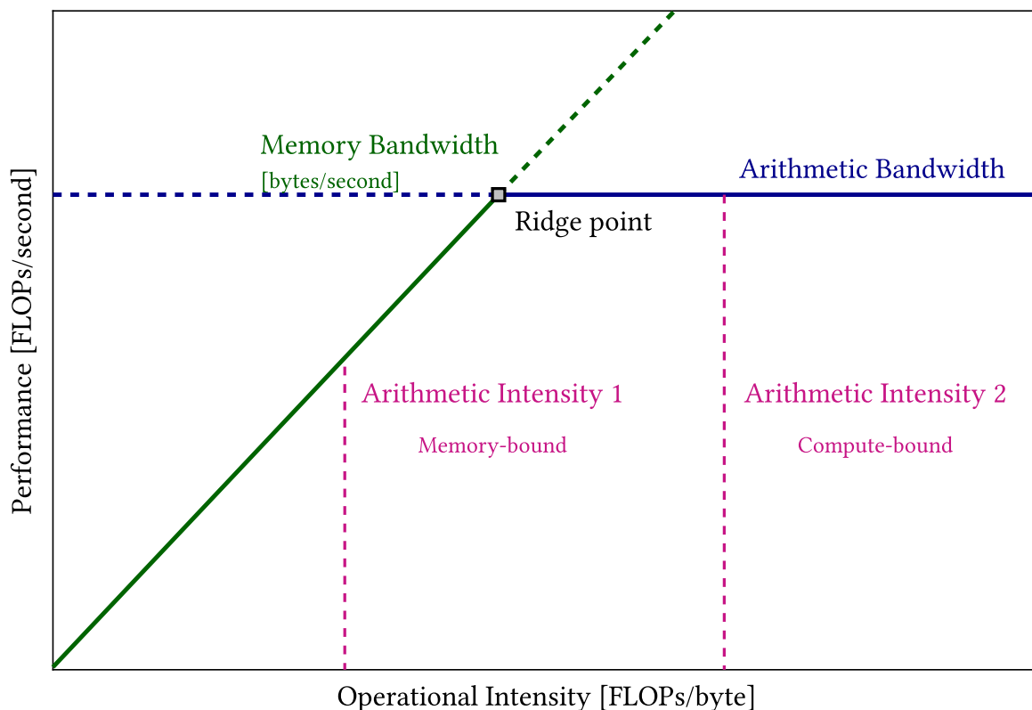
Fig. 1: Roofline model showing the relationship between arithmetic intensity and achievable performance. The memory bandwidth ceiling represents the GPU’s memory bandwidth limit, while the compute ceiling shows the maximum achievable TFLOPs. Kernels falling into the area to the left of the ridge point are memory-bound, while they are compute-bound if they fall into the right area.
