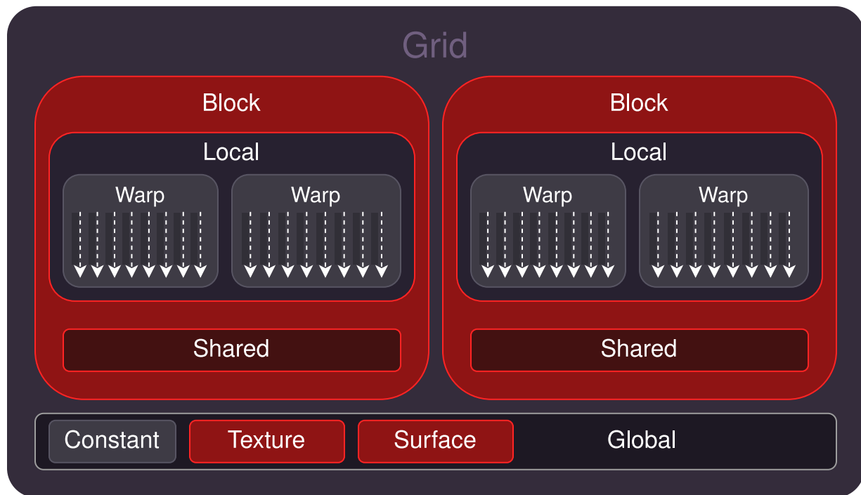
Fig. 5: Memory hierarchy.
